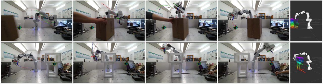
Fig. 15. PMMPI in dynamic obstacle avoidance scenarios: sudden obstacle appearance (top row) and obstacle left-right moving (bottom row). The robotic manipulator moves between two poses and arbitrary objects can serve as obstacles.
