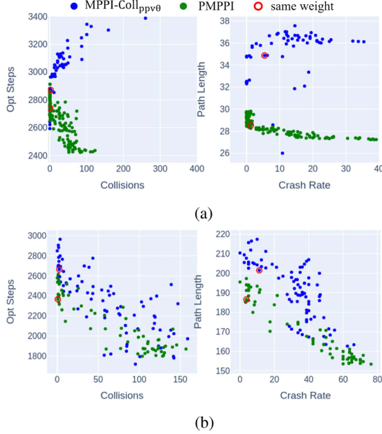
Fig. 11. Running time and collisions distribution, as well as path length and crash rate distribution for both algorithms in Task 1 and Task 3, respectively. (a) 2-D PointMass. (b) Franka.
