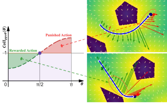
Fig. 6. GVM-SDF: The planned path (blue line) over 20 steps (white points). Arrows indicate gradients, with length representing potential values. Green arrows denote robot velocity aligned with the SDF gradient, corresponding actions should be encouraged. Red arrows indicate the opposite.
