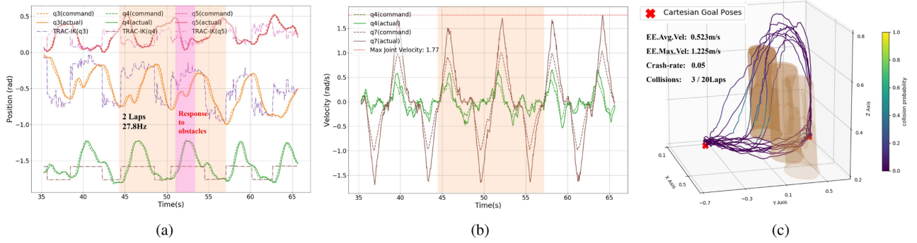
Fig. 14. Joint positions, velocities, and EE trajectories in sudden obstacle appearance scenario (see Fig. 15, top row). (a) Joints positions. (b) Joints velocities. (c) EE trajectories.
