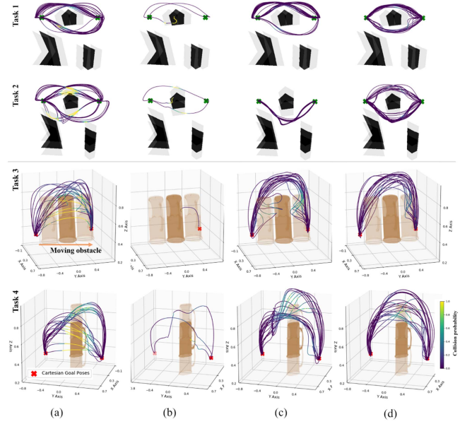
Fig. 9. Comparison of trajectories generated by the MPPI, utilizing Coll_p , Coll_{pv} , and Coll_{ppv\theta} , and the PMMPI. (a) Coll_p . (b) Coll_{pv} . (c) Coll_{ppv\theta} . (d) PMMPI.
