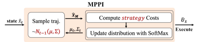
Fig. 2. MPPI architecture.
