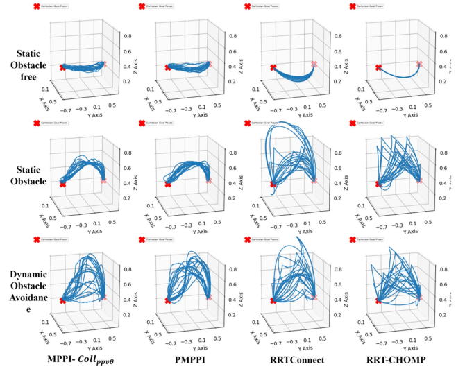
Fig. 13. EE. Trajectory visualization for different methods in three experimental scenarios.
