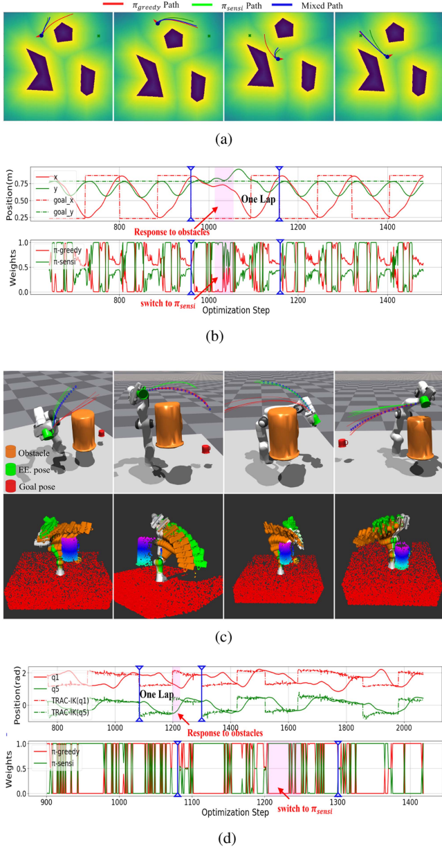
Fig. 8. Illustration of the PMMPI's performance over one lap for 2-D PointMass (Task 1) and Franka (Task 3), with recorded positions and weight distributions. Bottom row of (c) are environment point clouds and joints sequences, with orange and green trajectories representing \pi_{greedy} and \pi_{sensi} plans. (a) PMMPI performance (one lap) for 2-D PointMass. (b) Positions and weight distribution for 2-D PointMass. (c) PMMPI performance (one lap) for Franka. (d) Positions and weight distribution for Franka.
