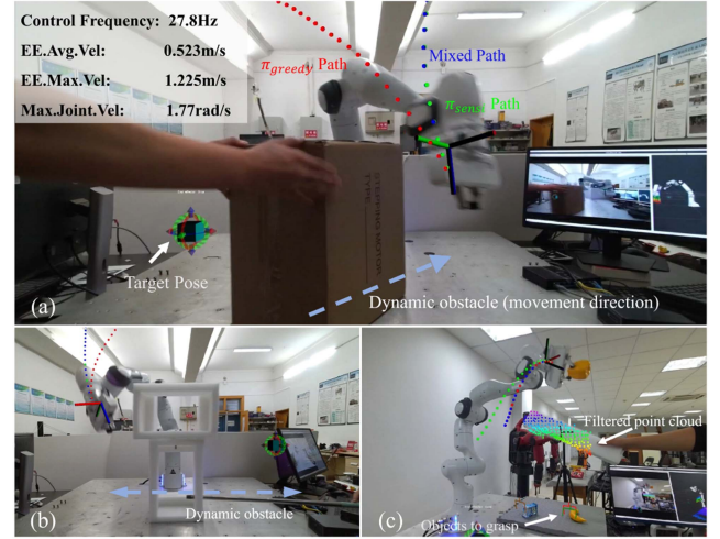
Fig. 1. Scenarios of dynamic obstacle avoidance using the PMPPI framework. (a) Obstacle suddenly appears in the robot's path, testing real-time response to unexpected events. (b) Dynamic obstacle crosses the workspace, requiring immediate trajectory adjustment. (c) Obstacle interferes with a pick-and-place task, evaluating the system's ability to balance task completion and dynamic avoidance.
