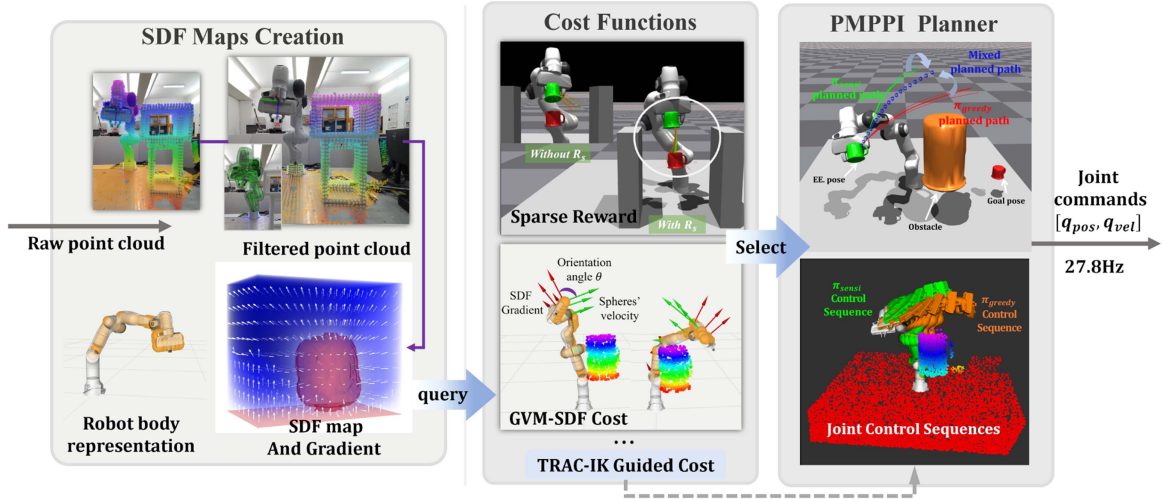
Fig. 3. Architecture overview of the PMMPI.
