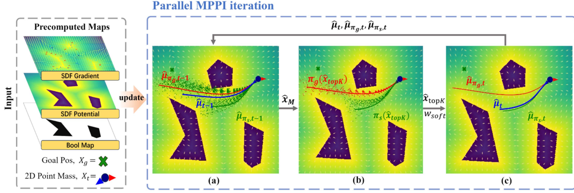
Fig. 5. Illustration of one PMMPI iteration using a 2-D PointMass with red (gradient) and blue (velocity) arrows. Background: SDF gradient and potential maps overlaid, updated in real time. Scattered points: Trajectories from the PMMPI sampling. (a) Sample trajs. \hat{x}_M . (b) Evaluate different policies. (c) Mixed \hat{\mu}_t update.
