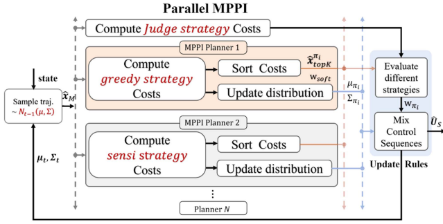
Fig. 4. PMPPI Architecture simplifies optimization by concurrently running multiple MPPI planners with different strategies, requiring only one sampling step per iteration.
