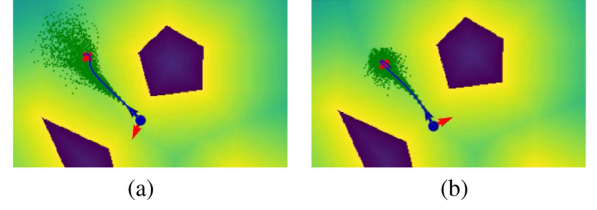
Fig. 7. Sparse reward illustration. (a) Without R_s(\text{dist}) . (b) With R_s(\text{dist}) .
